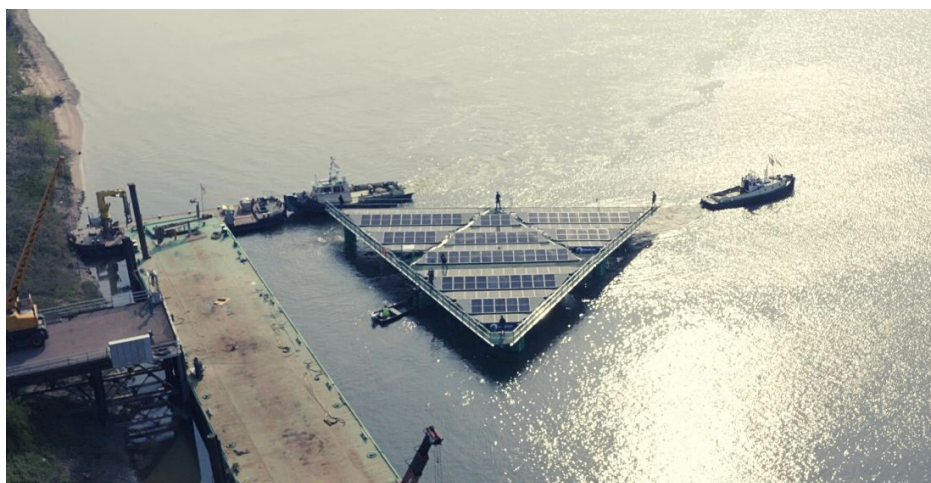
The SolarDuck project Demonstrator floats at IJzendoorn in the Netherlands and delivers energy to the grid.
